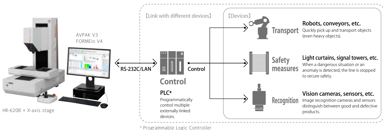
Example of Rockwell hardness testing machine automation on a production line
